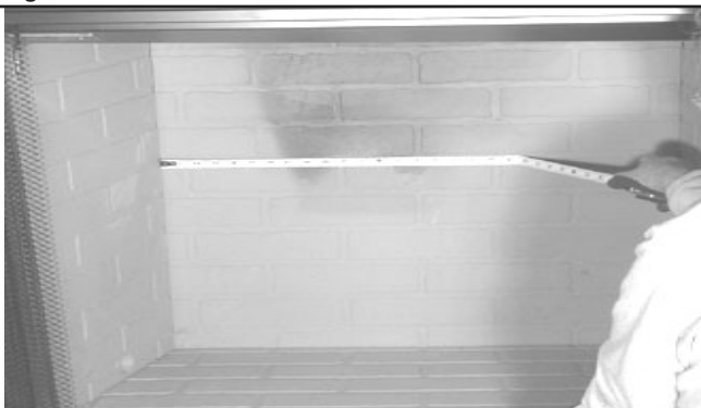
Figure 1 Measure Firebox
